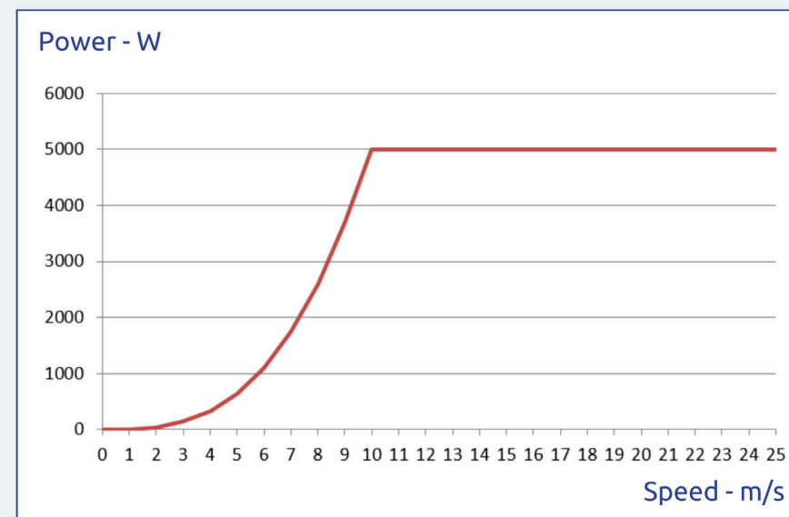
SoyutWind 5 kW Power Curve
