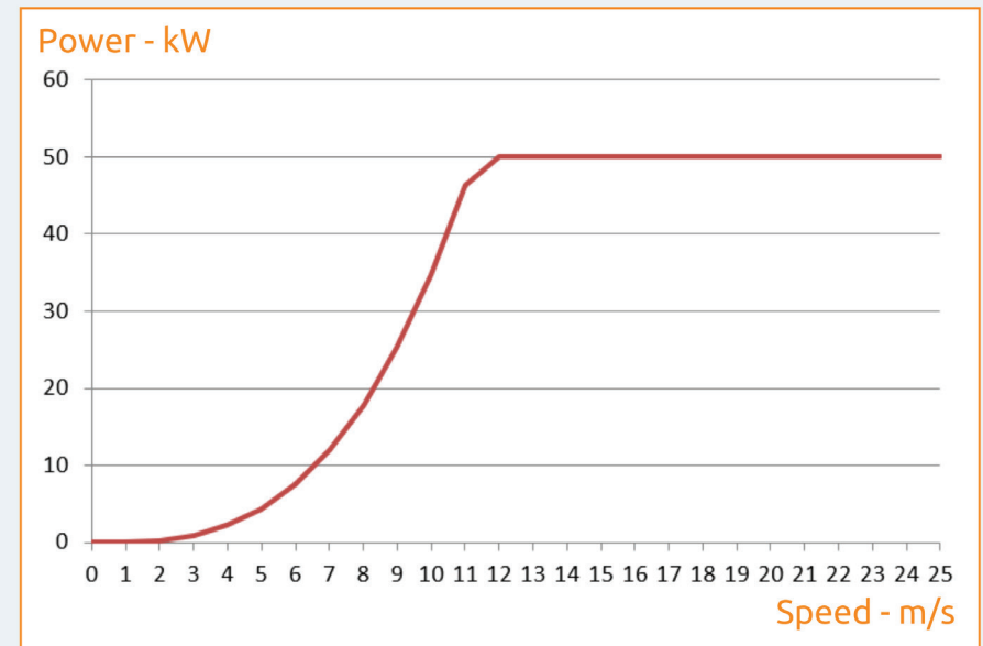
SoyutWind 50 kW Power Curve
