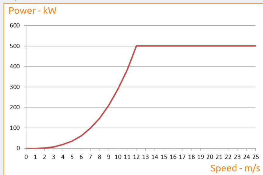
SoyutWind 500 kW Power Curve
