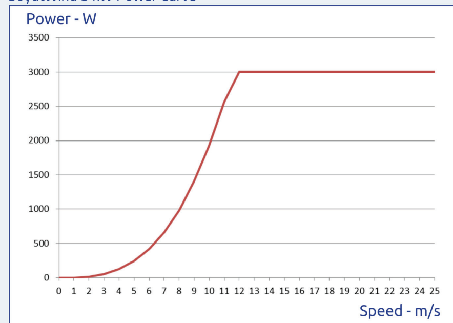
SoyutWind 3 kW Power Curve
