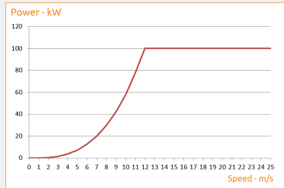
SoyutWind 100 KW Power Curve
